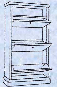
Art. 6826 Scarpiera 3 ribalte liscia Shoe cabinet L 77 H 118 P 20
